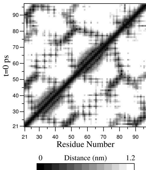
Fig. 5.57: A minimum distance matrix for a peptide 168 (page 576).
