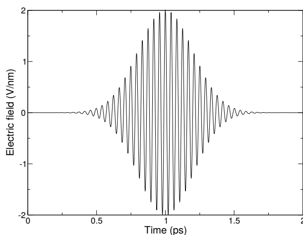
Fig. 5.48: A simulated laser pulse in GROMACS.
