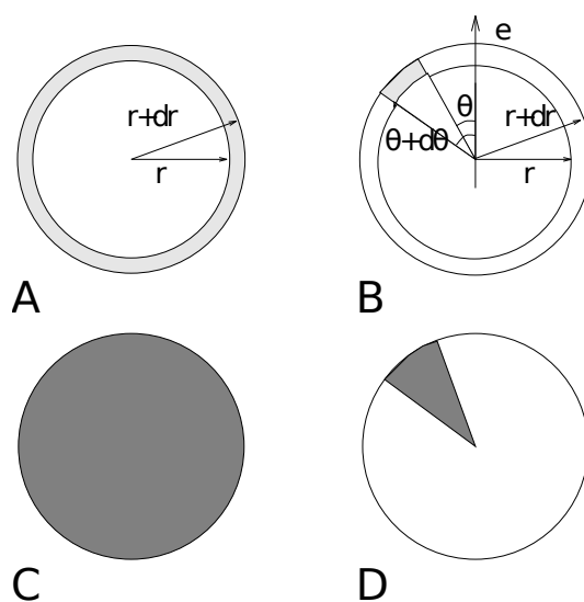
Fig. 5.52: Definition of slices in gmx rdf (page 244): A. g_{AB}(r) . B. g_{AB}(r, \theta) . The slices are colored gray. C. Normalization \langle \rho_B \rangle_{local} . D. Normalization \langle \rho_B \rangle_{local, \theta} . Normalization volumes are colored gray.
