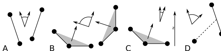
Fig. 5.56: Angle options of gmx gangle (page 186): A. Angle between two vectors. B. Angle between two planes. C. Angle between a vector and the z axis. D. Angle between a vector and the normal of a sphere. Also other combinations are supported: planes and vectors can be used interchangeably.
