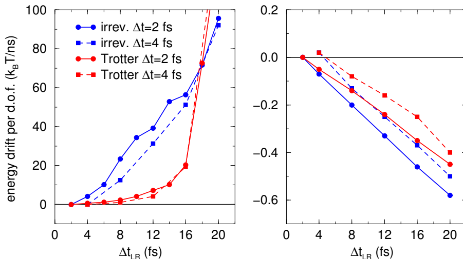
Figure 3.8: Energy drift per degree of freedom in SPC/E water with twin-range cut-offs for reaction field (left) and Lennard-Jones interaction (right) as a function of the long-range time step length for the irreversible “GROMOS” scheme and a reversible Trotter scheme.
